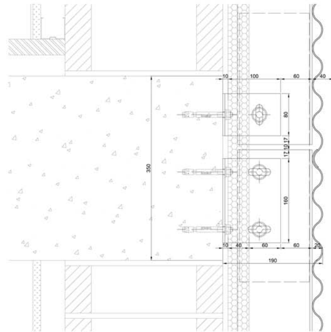
DETALLE VERTICAL V-02.MO
