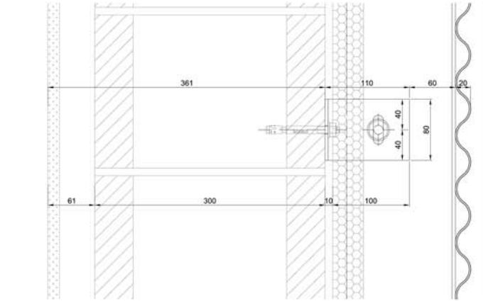
DETALLE VERTICAL V-01.MO
